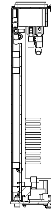
SECTION B-B
